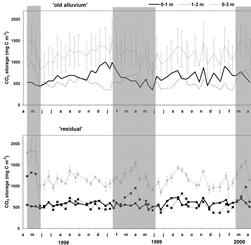
Figure 2. Bi-weekly measurements of soil CO 2 storage in 0–1 m, 1–3 m and 0–3 m depth. Means ( \pm standard error) are given ( n = 3 ). The shaded areas mark the drier season; white background is the wet season.
