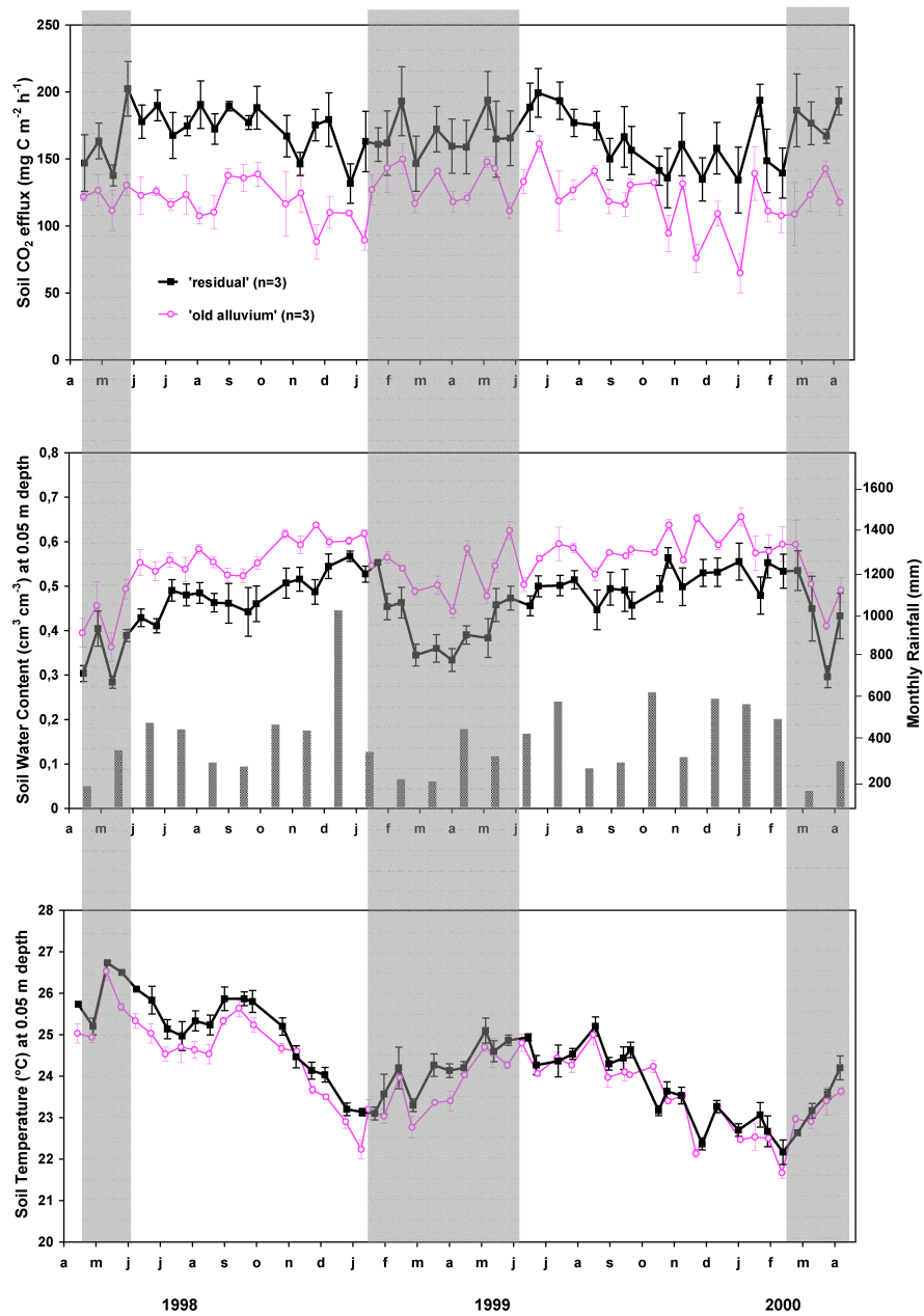
Figure 1. Bi-weekly measurements of soil CO 2 efflux, soil water content and soil temperature at 0.05 m depth. Each point is the mean of three sites (for soil respiration with 8 chamber measurements at each site). Error bars represent \pm standard error of the mean. The shaded areas mark the drier season; white background is the wet season.
