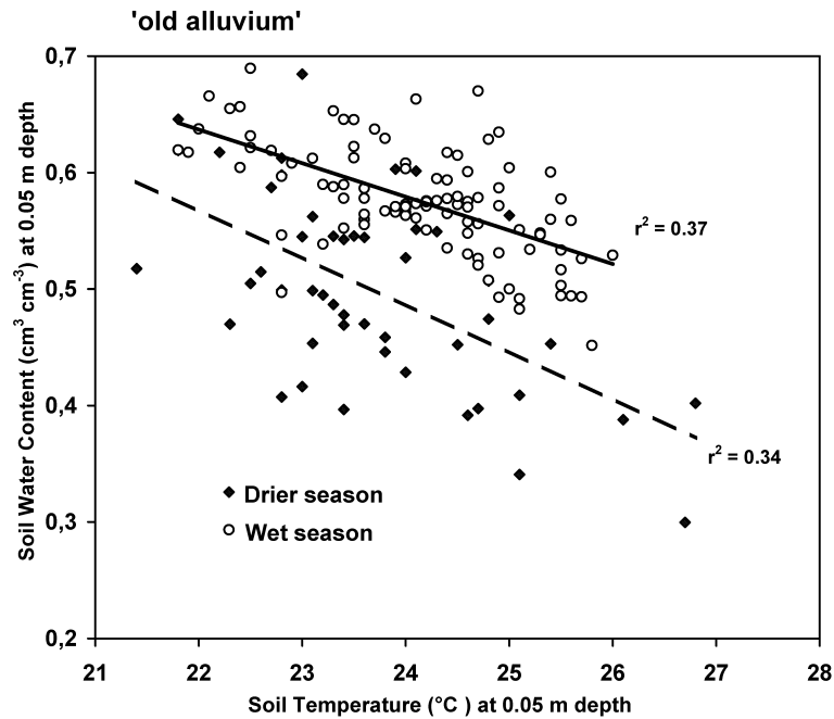
Figure 4. Covariation of soil temperature with soil water content at 0.05 m depth for 'old alluvium'. Each point represents individual soil temperature and soil water measurements made at all 'old alluvium' sites on a given date.
