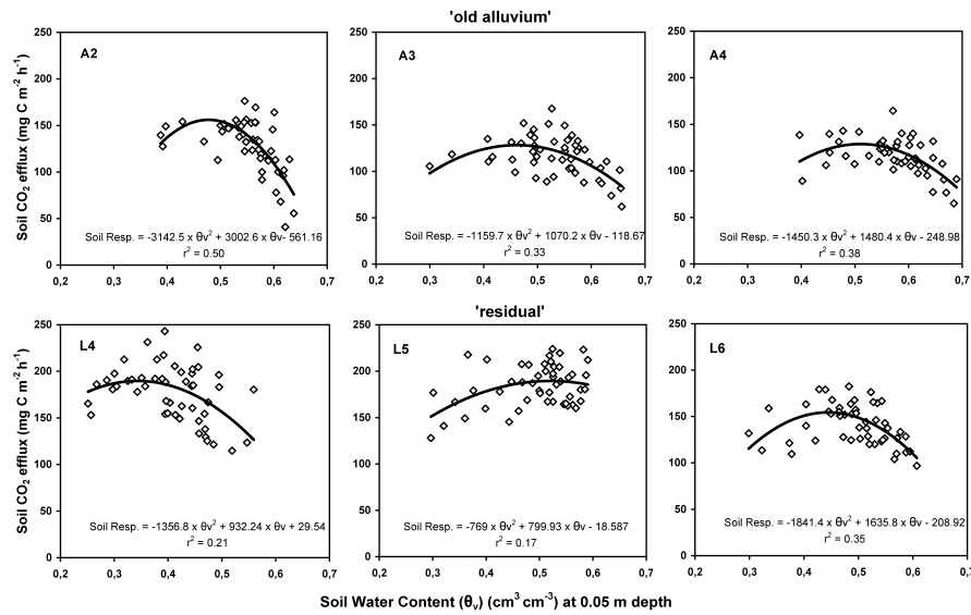
Figure 3. Relationship between soil water content and soil \text{CO}_2 efflux. Each estimate of soil \text{CO}_2 efflux is a mean of 8 chamber measurements and one soil water measurement at 0.05 m depth made on a given date.
